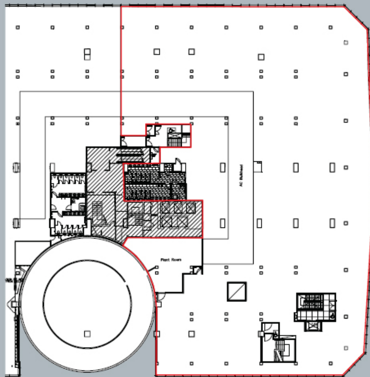
FIRST FLOOR OFFICE SPACE
